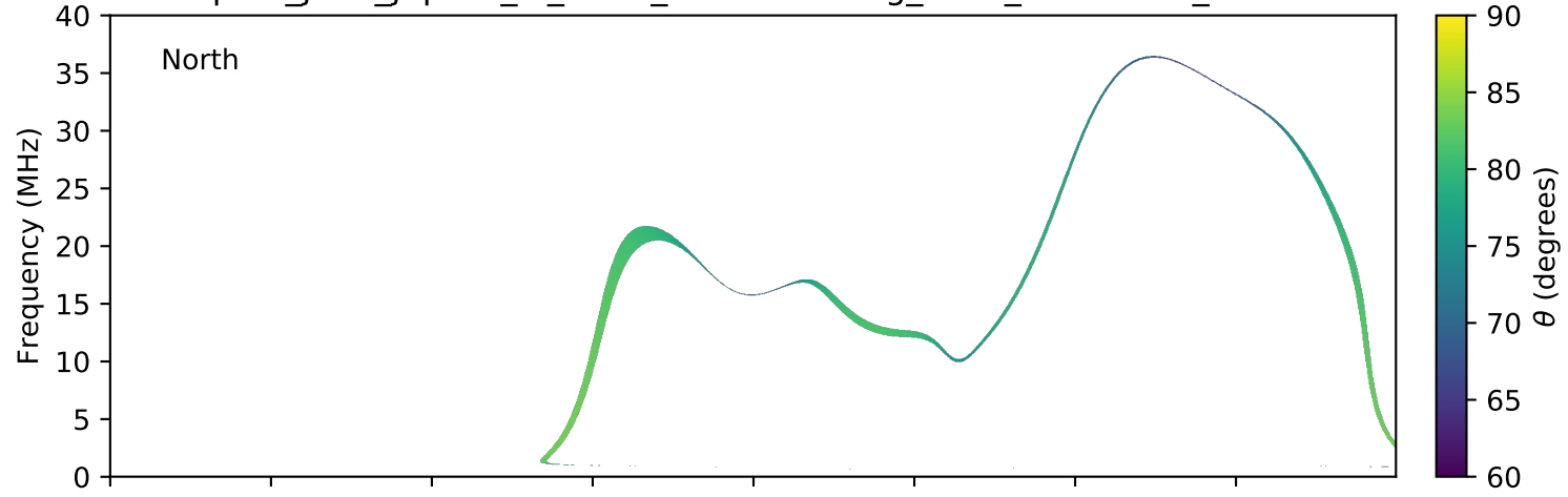
expres_juno_jupiter_io_isaac_lossc-wid1deg_3kev_20180805_v01.cdf
