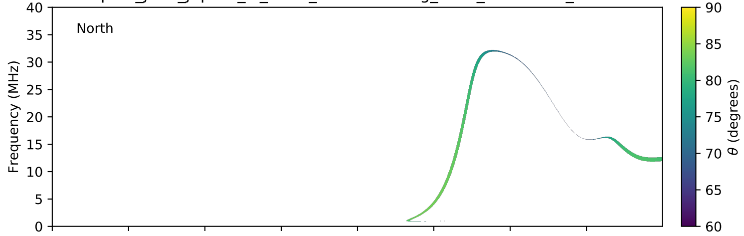
expres_juno_jupiter_io_isaac_lossc-wid1deg_3kev_20180803_v01.cdf
