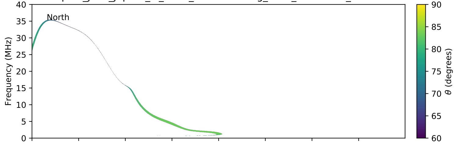
expres_juno_jupiter_io_isaac_lossc-wid1deg_3kev_20180802_v01.cdf
