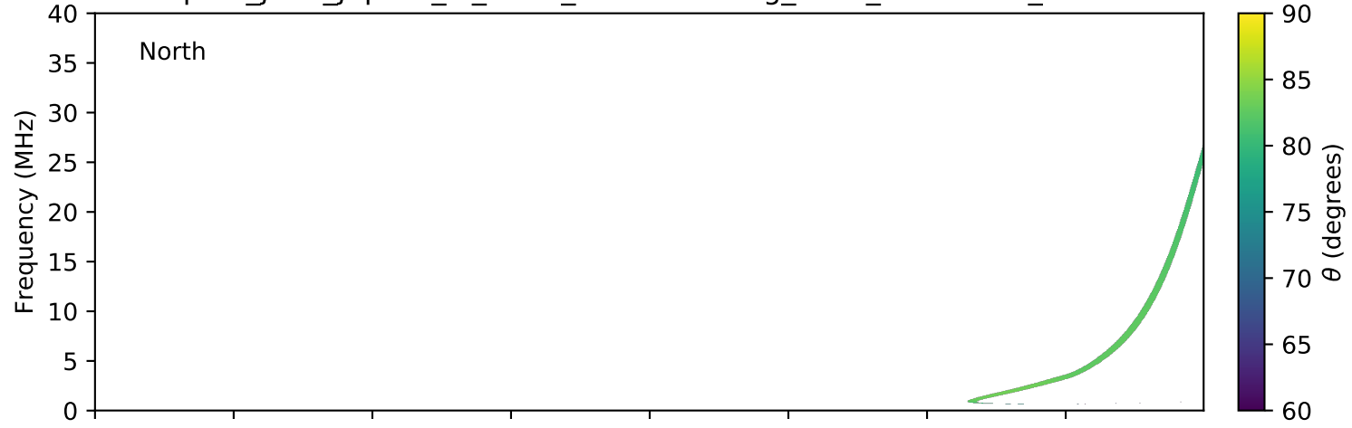
expres_juno_jupiter_io_isaac_lossc-wid1deg_3kev_20180801_v01.cdf
