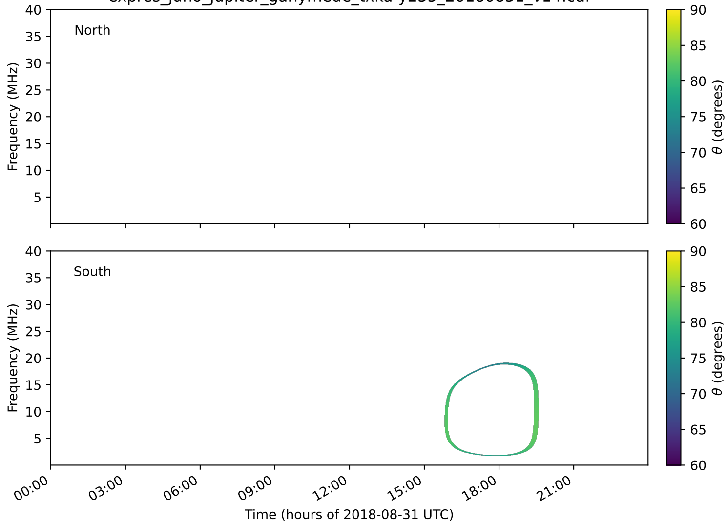
expres_juno_jupiter_ganymede_txka-y235_20180831_v14.cdf
