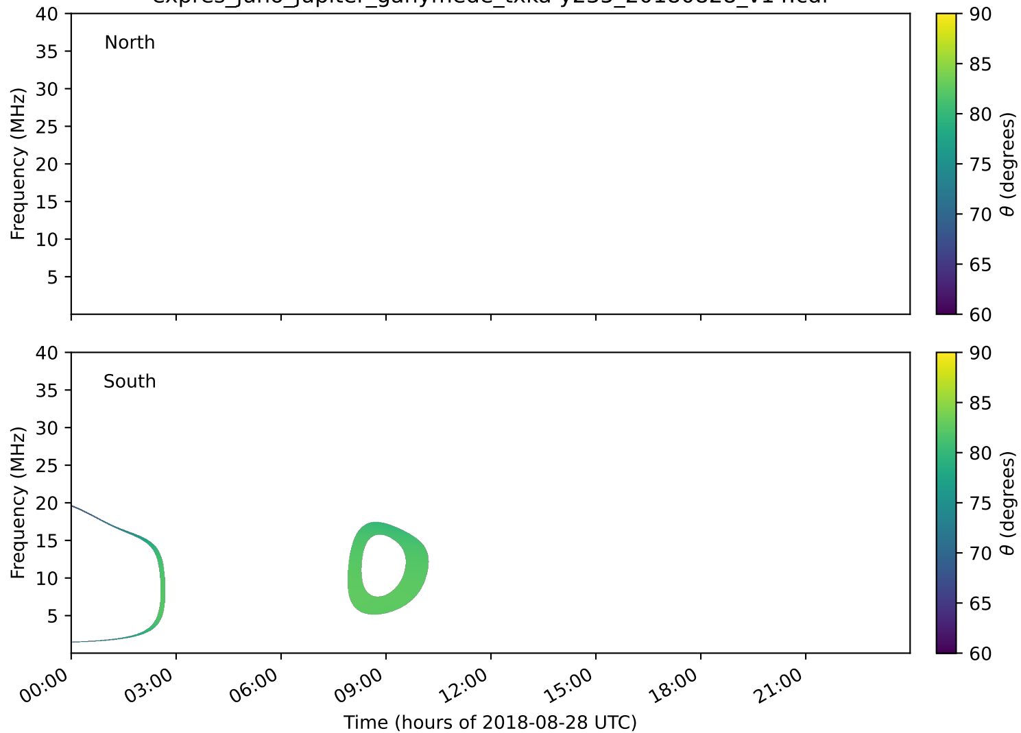
expres_juno_jupiter_ganymede_txka-y235_20180828_v14.cdf
