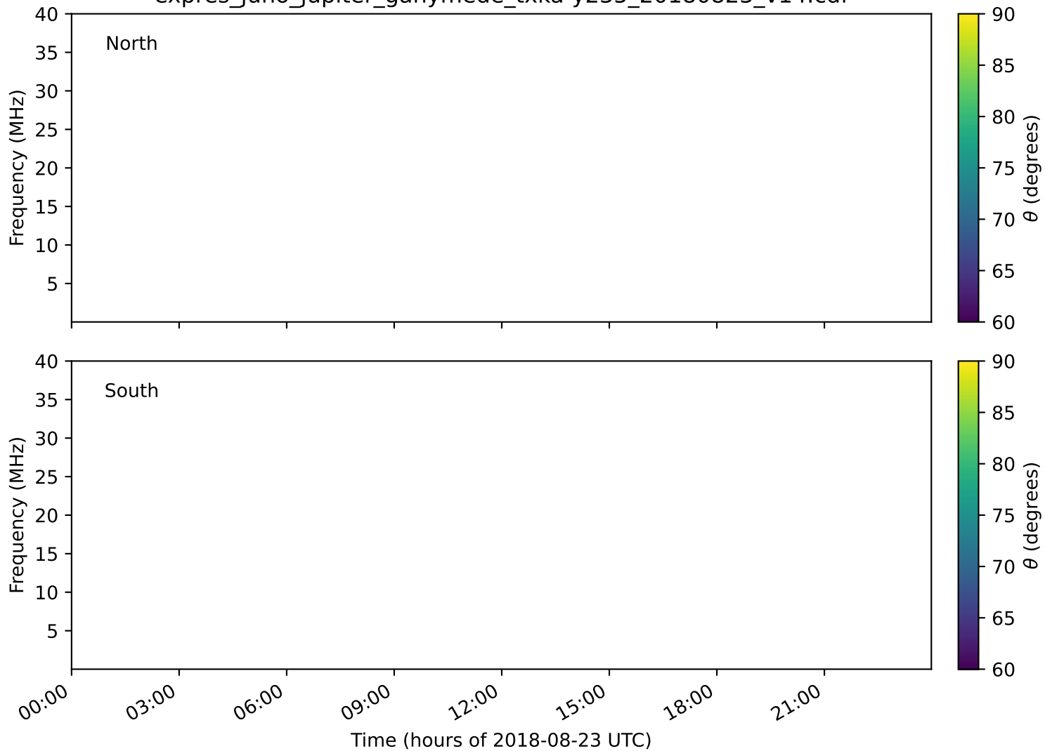
expres_juno_jupiter_ganymede_txka-y235_20180823_v14.cdf
