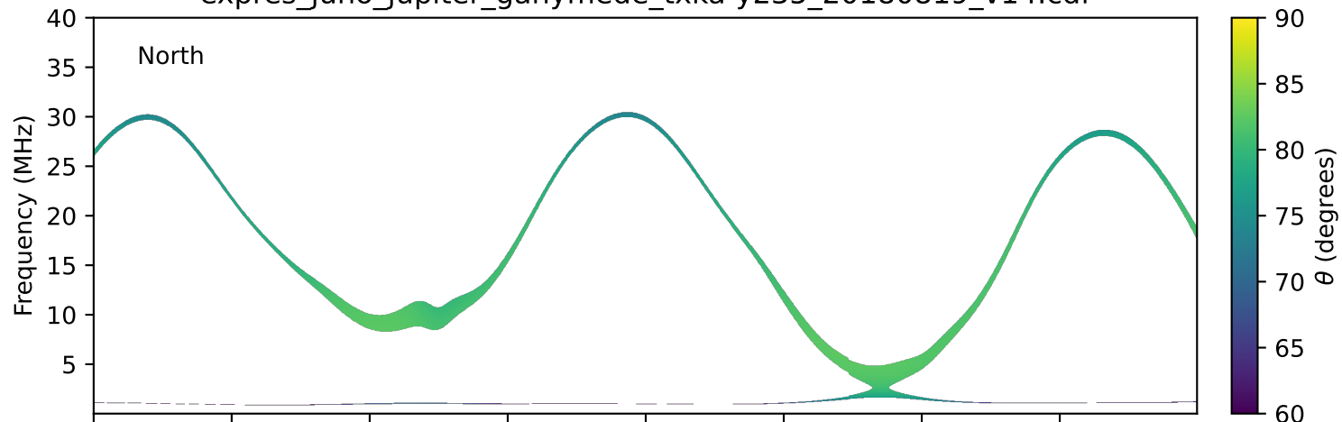
expres_juno_jupiter_ganymede_txka-y235_20180819_v14.cdf
