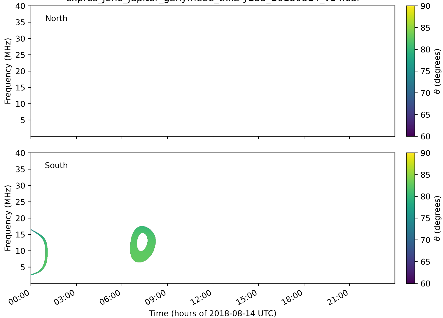
expres_juno_jupiter_ganymede_txka-y235_20180814_v14.cdf
