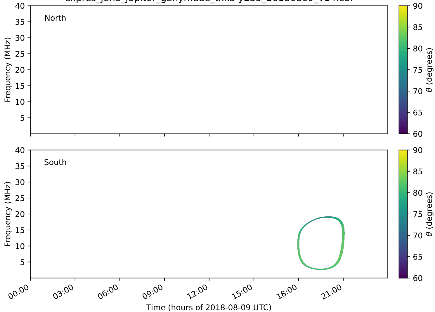
expres_juno_jupiter_ganymede_txka-y235_20180809_v14.cdf
