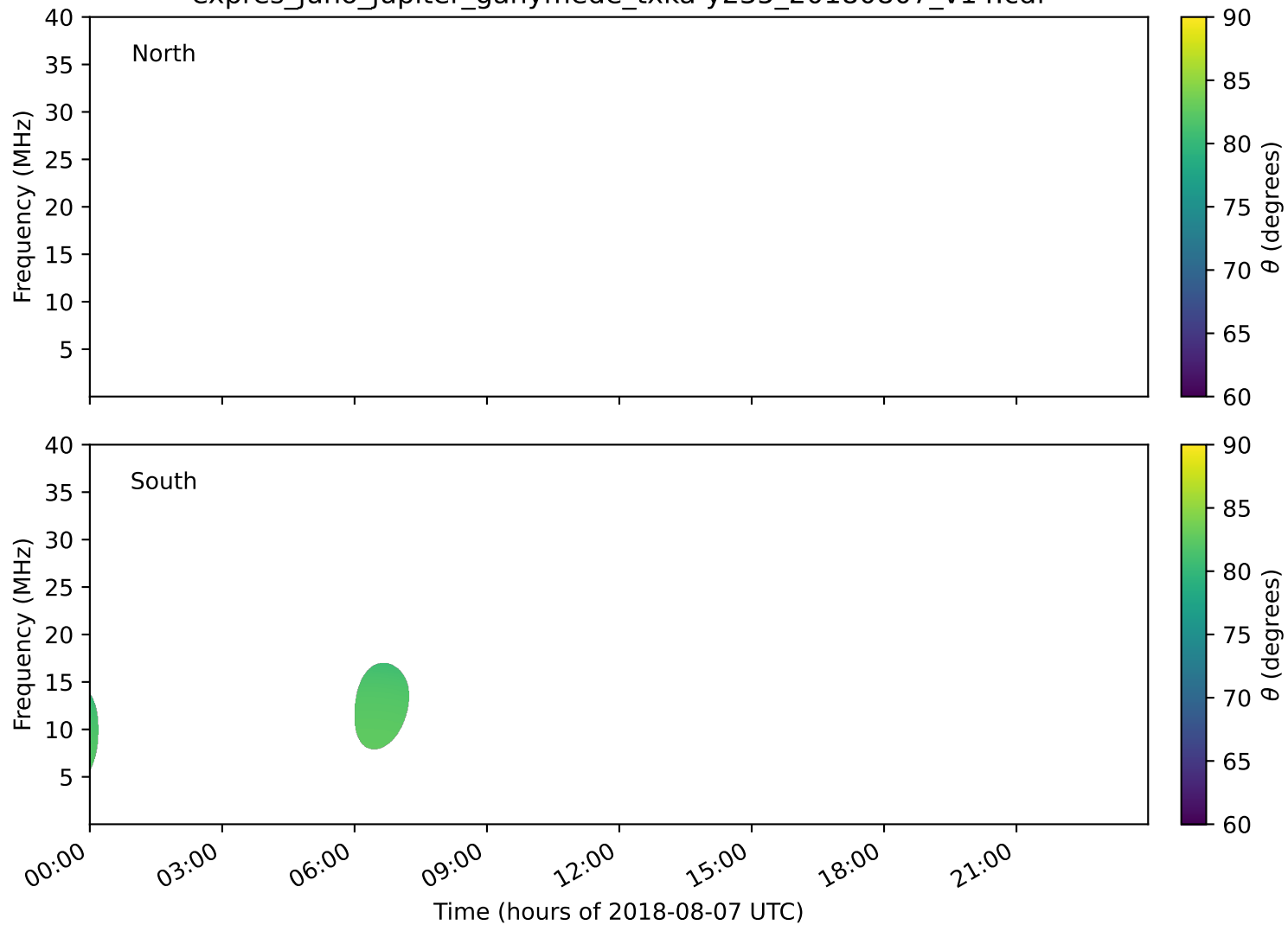
expres_juno_jupiter_ganymede_txka-y235_20180807_v14.cdf
