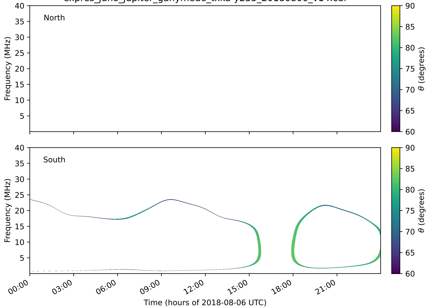
expres_juno_jupiter_ganymede_txka-y235_20180806_v14.cdf
