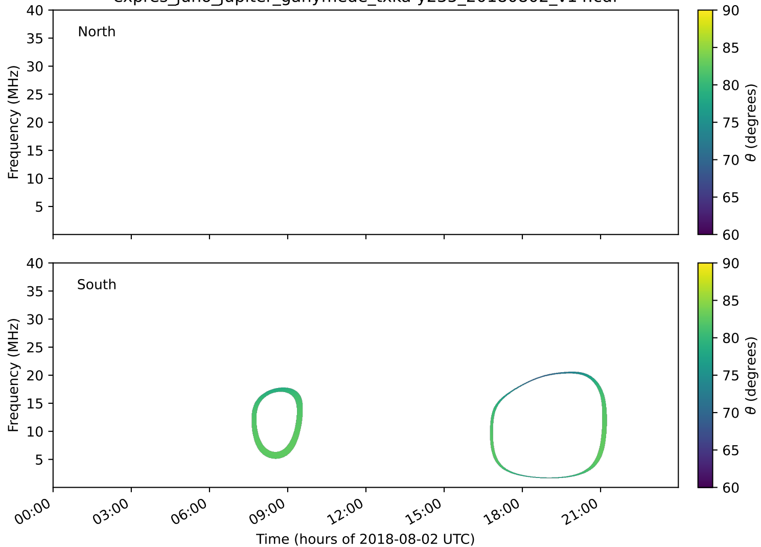
expres_juno_jupiter_ganymede_txka-y235_20180802_v14.cdf
