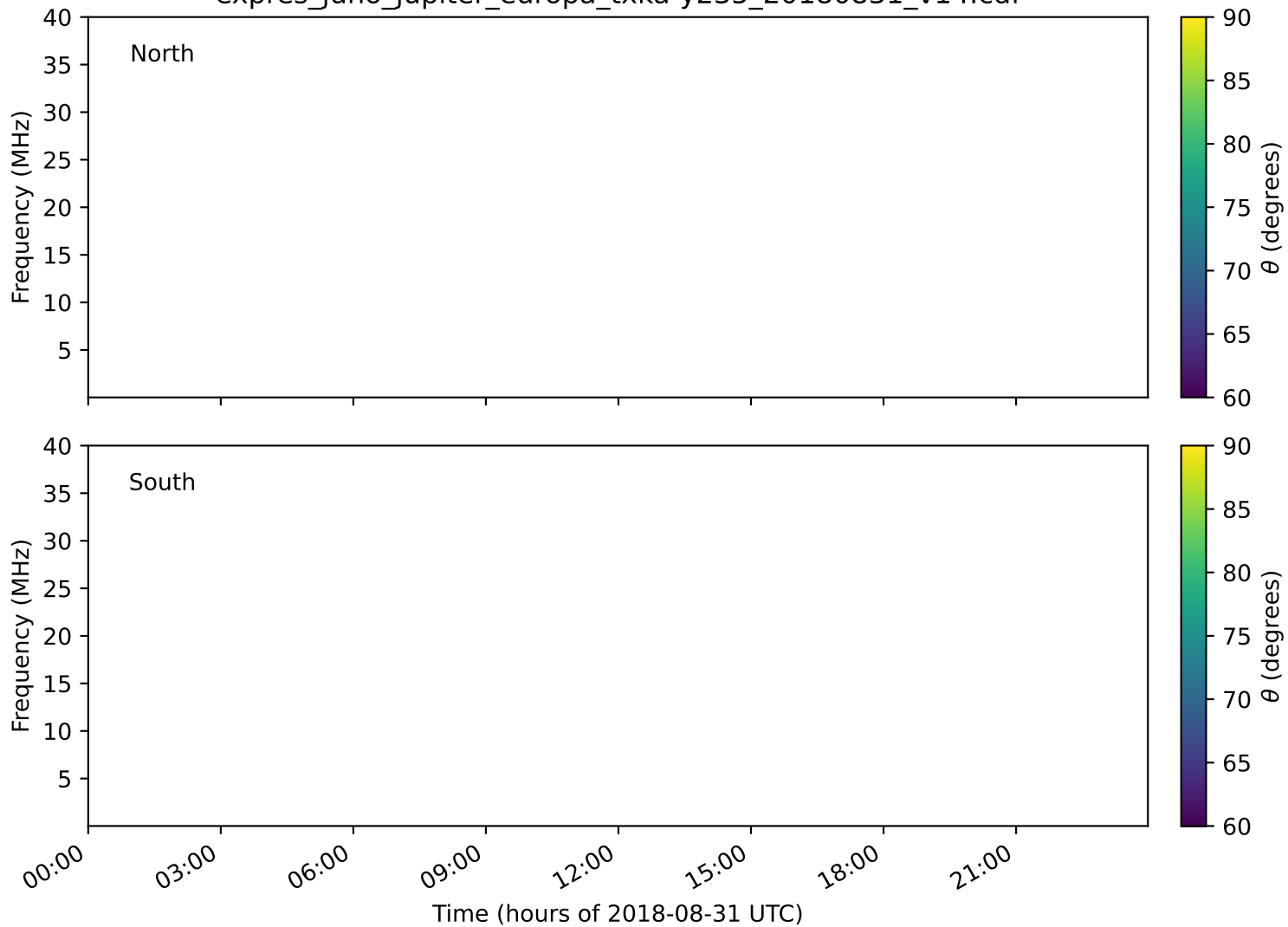
expres_juno_jupiter_europa_txka-y235_20180831_v14.cdf
