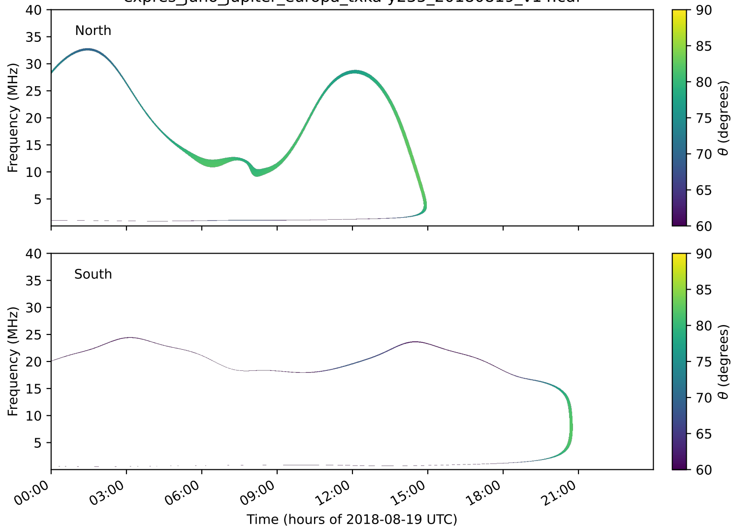
expres_juno_jupiter_europa_txka-y235_20180819_v14.cdf
