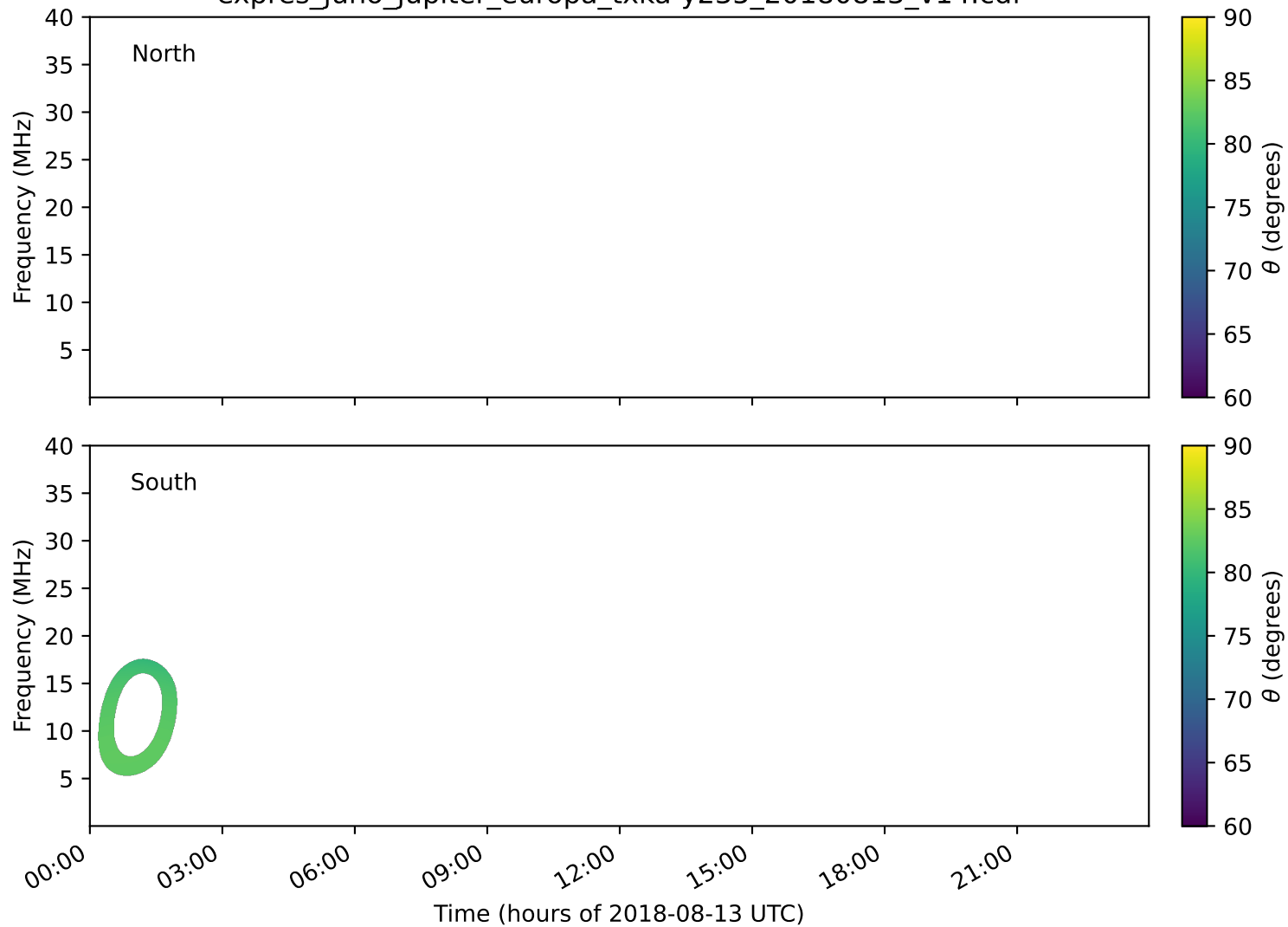
expres_juno_jupiter_europa_txka-y235_20180813_v14.cdf
