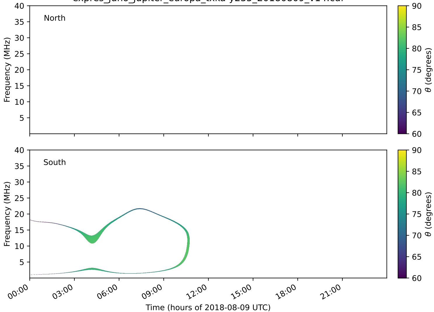
expres_juno_jupiter_europa_txka-y235_20180809_v14.cdf
