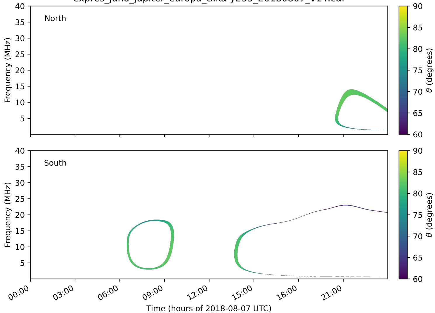
expres_juno_jupiter_europa_txka-y235_20180807_v14.cdf
