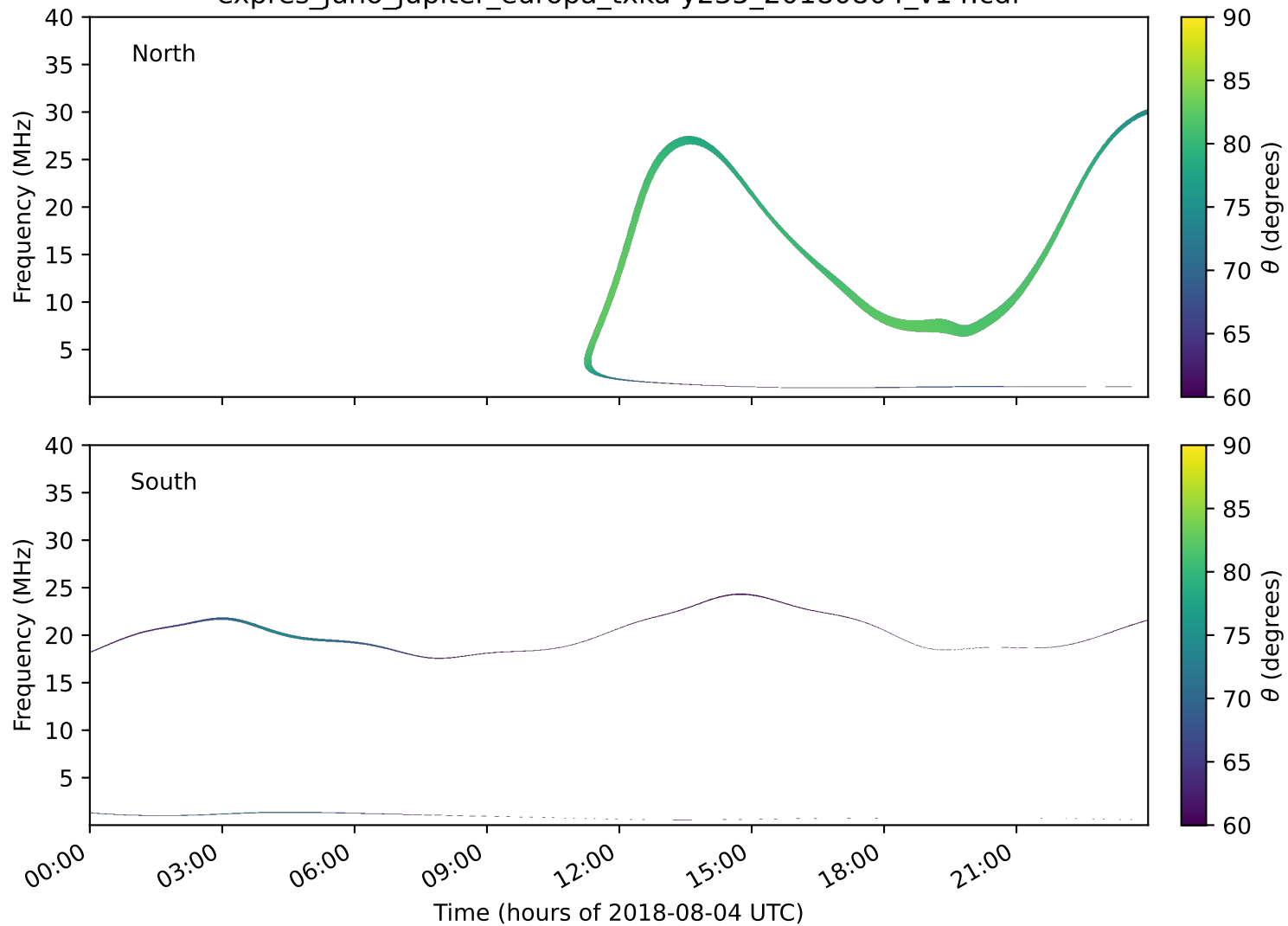
expres_juno_jupiter_europa_txka-y235_20180804_v14.cdf
