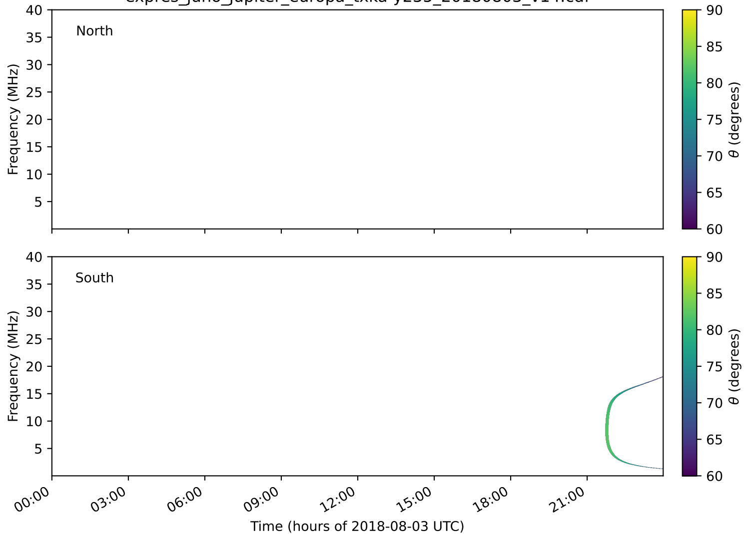
expres_juno_jupiter_europa_txka-y235_20180803_v14.cdf
