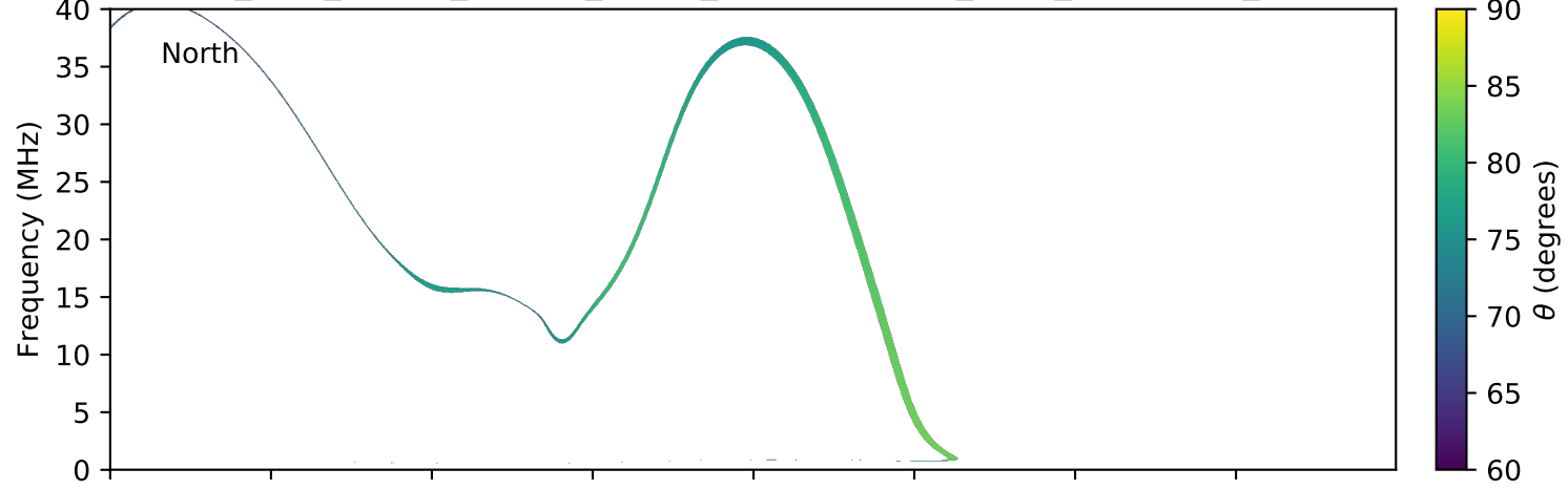
expres_juno_jupiter_europa_jrm09_lossc-wid1deg_3kev_20180831_v01.cdf
