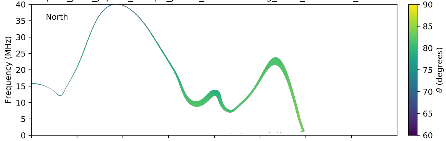
expres_juno_jupiter_europa_jrm09_lossc-wid1deg_3kev_20180830_v01.cdf
