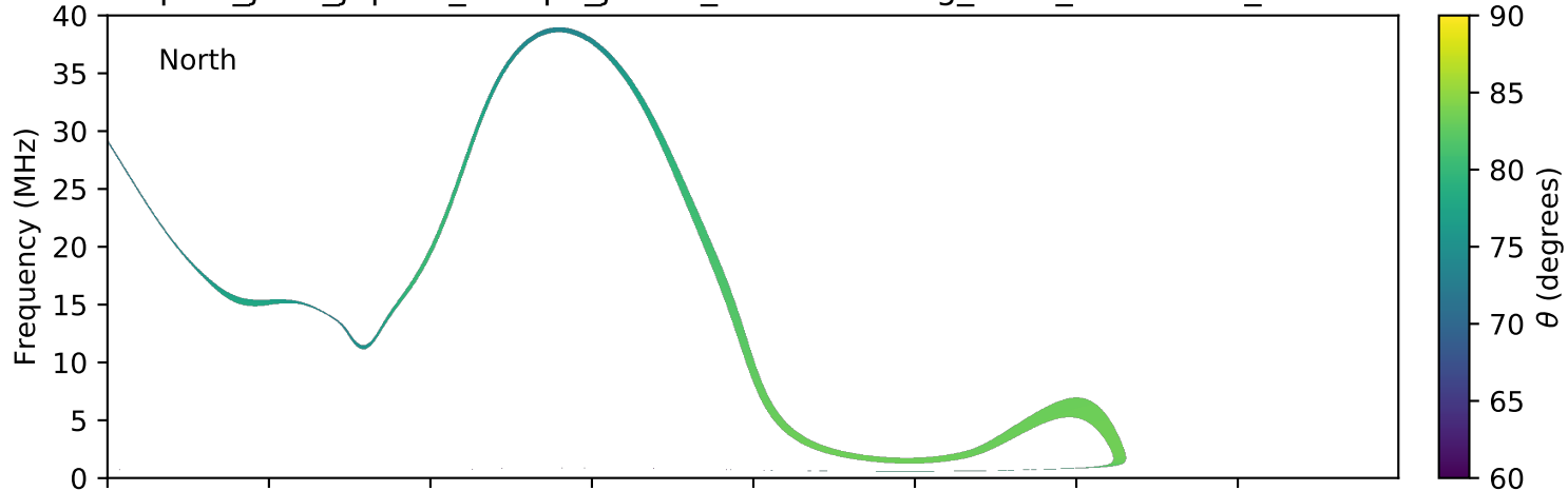
expres_juno_jupiter_europa_jrm09_lossc-wid1deg_3kev_20180827_v01.cdf
