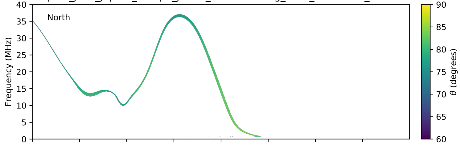
expres_juno_jupiter_europa_jrm09_lossc-wid1deg_3kev_20180822_v01.cdf
