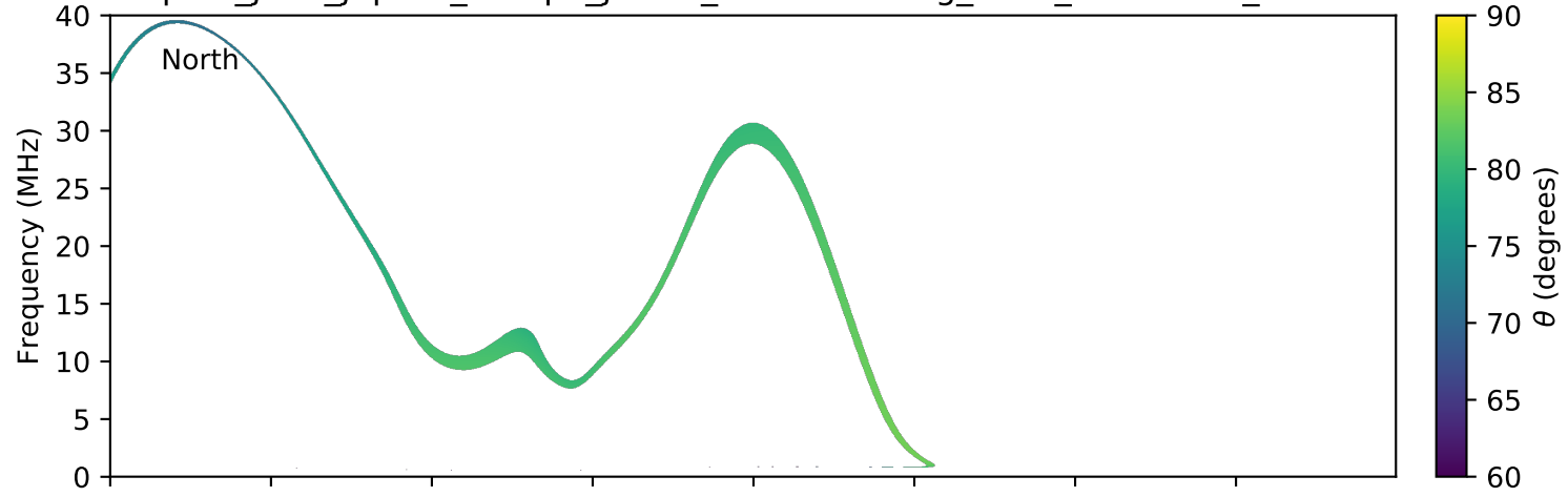
expres_juno_jupiter_europa_jrm09_lossc-wid1deg_3kev_20180819_v01.cdf
