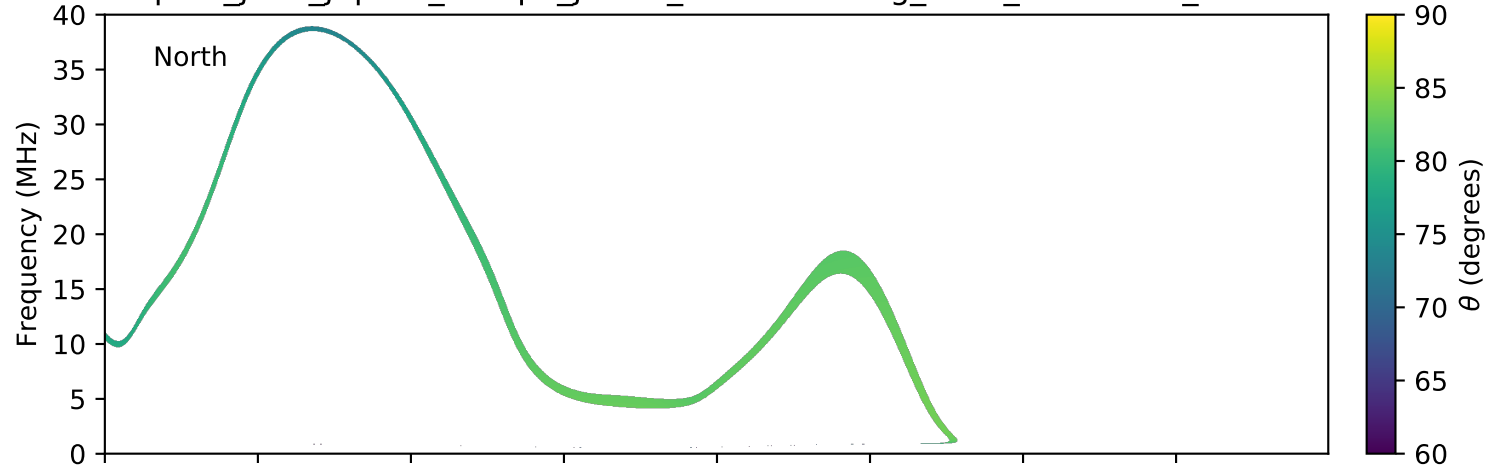
expres_juno_jupiter_europa_jrm09_lossc-wid1deg_3kev_20180816_v01.cdf
