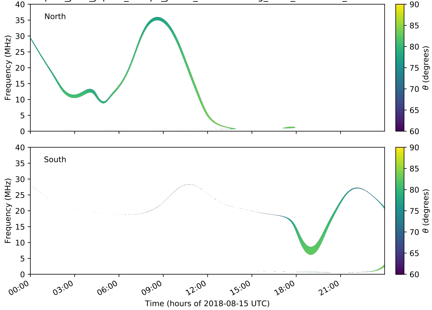
expres_juno_jupiter_europa_jrm09_lossc-wid1deg_3kev_20180815_v01.cdf
