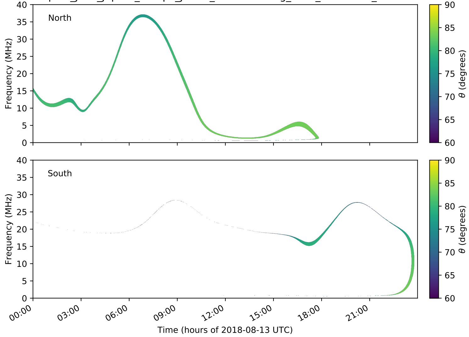
expres_juno_jupiter_europa_jrm09_lossc-wid1deg_3kev_20180813_v01.cdf
