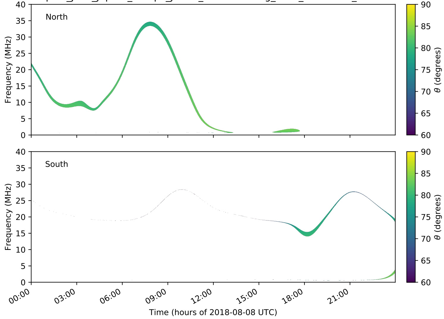
expres_juno_jupiter_europa_jrm09_lossc-wid1deg_3kev_20180808_v01.cdf
