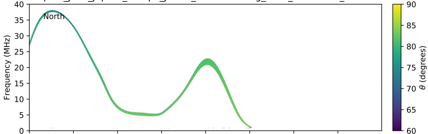
expres_juno_jupiter_europa_jrm09_lossc-wid1deg_3kev_20180807_v01.cdf
