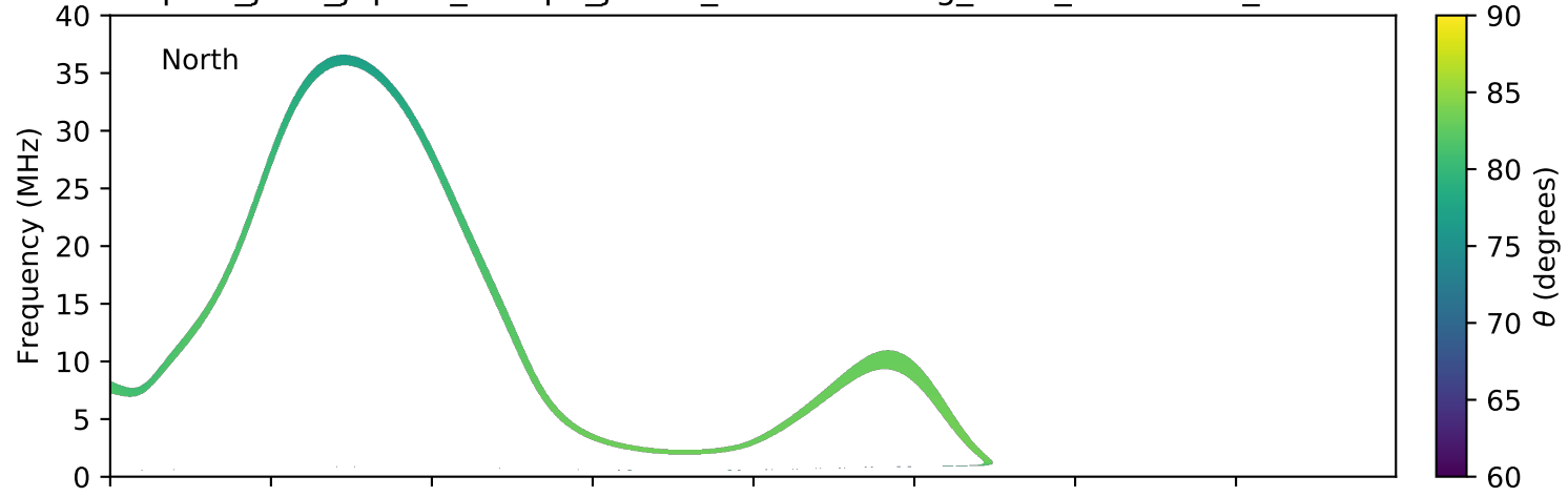
expres_juno_jupiter_europa_jrm09_lossc-wid1deg_3kev_20180804_v01.cdf
