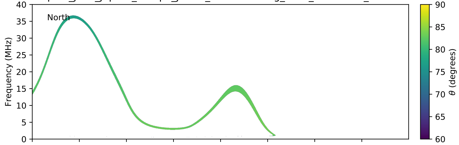
expres_juno_jupiter_europa_jrm09_lossc-wid1deg_3kev_20180802_v01.cdf
