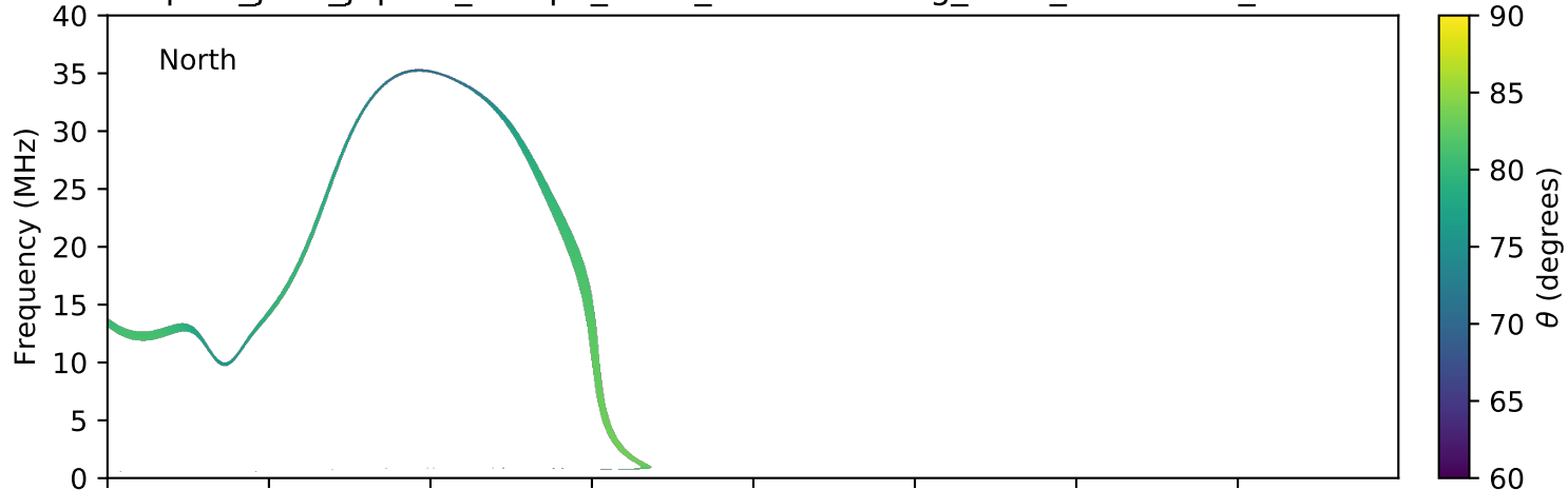
expres_juno_jupiter_europa_isaac_lossc-wid1deg_3kev_20180830_v01.cdf
