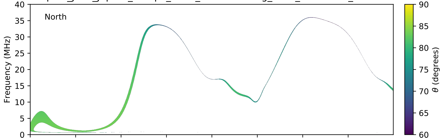
expres_juno_jupiter_europa_isaac_lossc-wid1deg_3kev_20180829_v01.cdf
