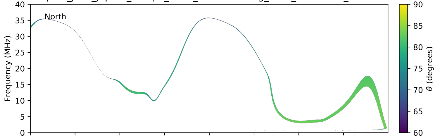
expres_juno_jupiter_europa_isaac_lossc-wid1deg_3kev_20180826_v01.cdf
