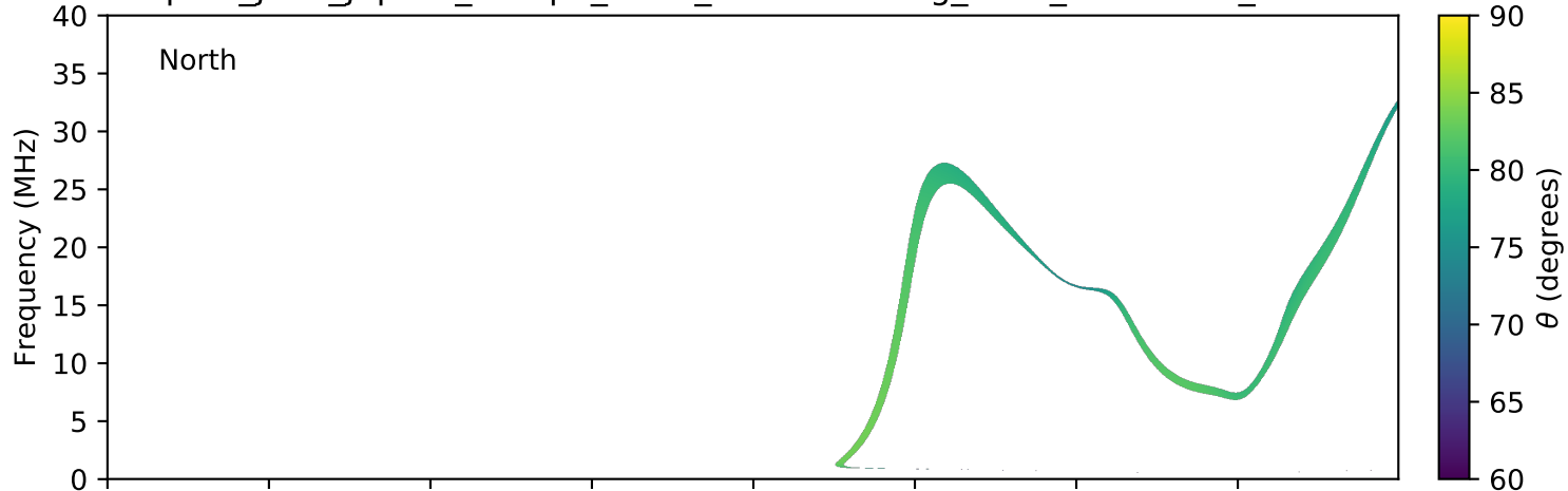
expres_juno_jupiter_europa_isaac_lossc-wid1deg_3kev_20180825_v01.cdf
