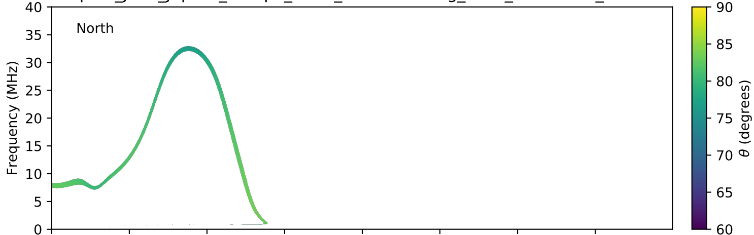
expres_juno_jupiter_europa_isaac_lossc-wid1deg_3kev_20180823_v01.cdf
