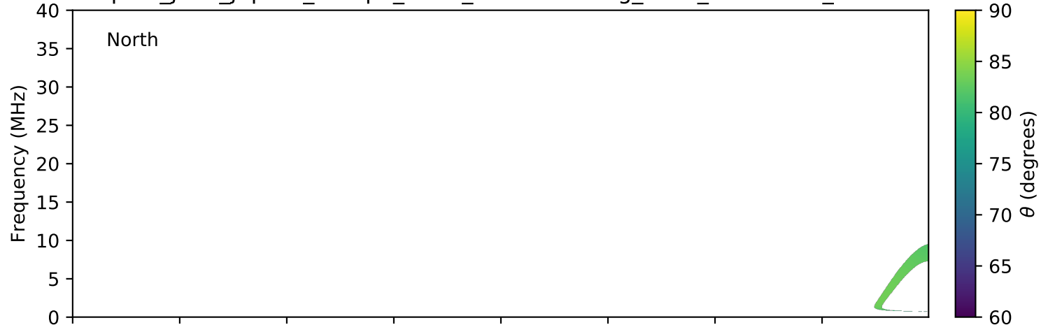
expres_juno_jupiter_europa_isaac_lossc-wid1deg_3kev_20180821_v01.cdf
