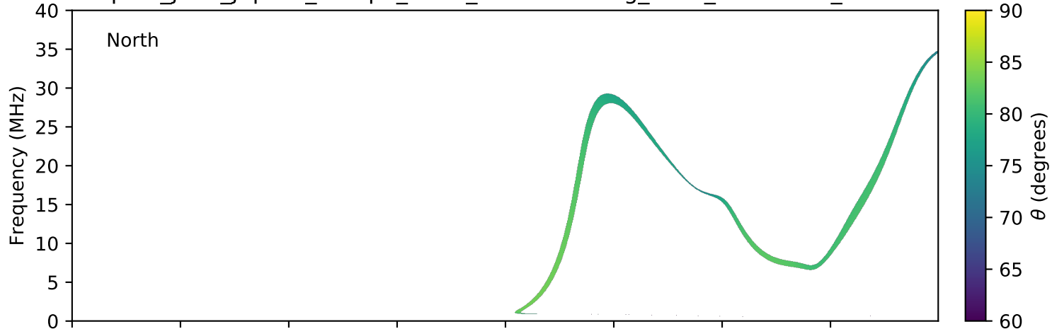
expres_juno_jupiter_europa_isaac_lossc-wid1deg_3kev_20180818_v01.cdf
