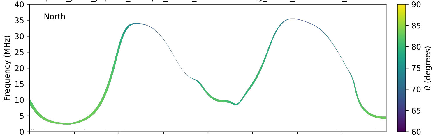
expres_juno_jupiter_europa_isaac_lossc-wid1deg_3kev_20180815_v01.cdf
