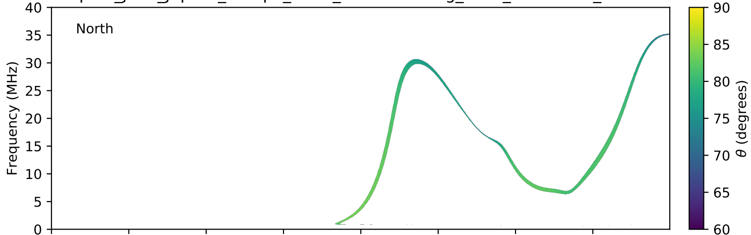
expres_juno_jupiter_europa_isaac_lossc-wid1deg_3kev_20180811_v01.cdf
