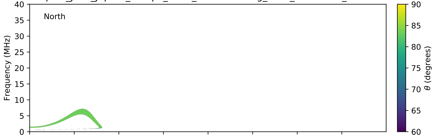
expres_juno_jupiter_europa_isaac_lossc-wid1deg_3kev_20180809_v01.cdf
