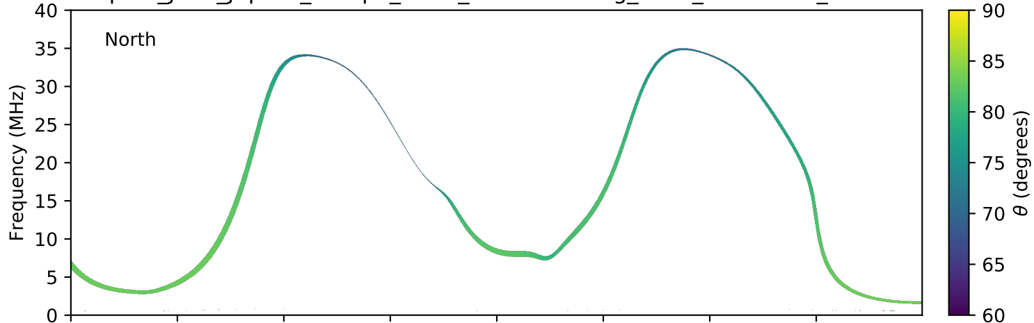
expres_juno_jupiter_europa_isaac_lossc-wid1deg_3kev_20180808_v01.cdf
