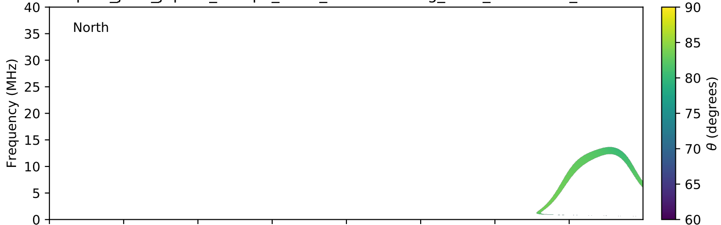
expres_juno_jupiter_europa_isaac_lossc-wid1deg_3kev_20180807_v01.cdf
