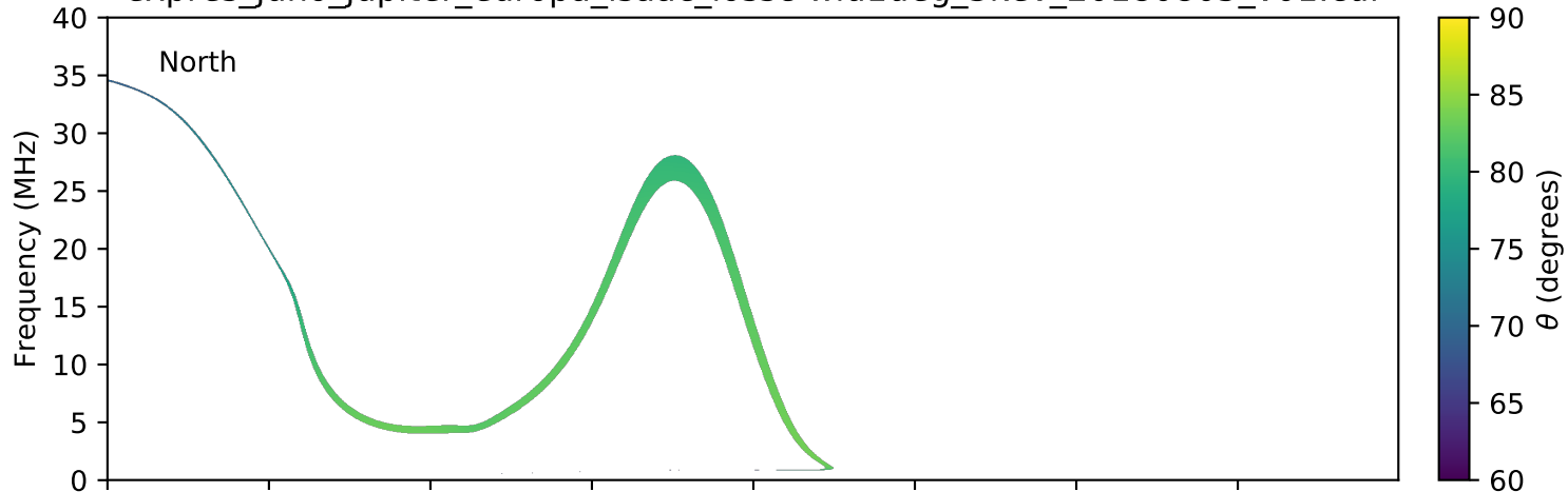
expres_juno_jupiter_europa_isaac_lossc-wid1deg_3kev_20180805_v01.cdf
