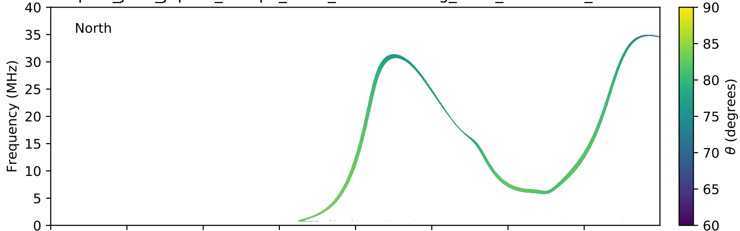
expres_juno_jupiter_europa_isaac_lossc-wid1deg_3kev_20180804_v01.cdf
