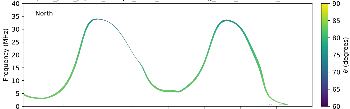
expres_juno_jupiter_europa_isaac_lossc-wid1deg_3kev_20180801_v01.cdf
