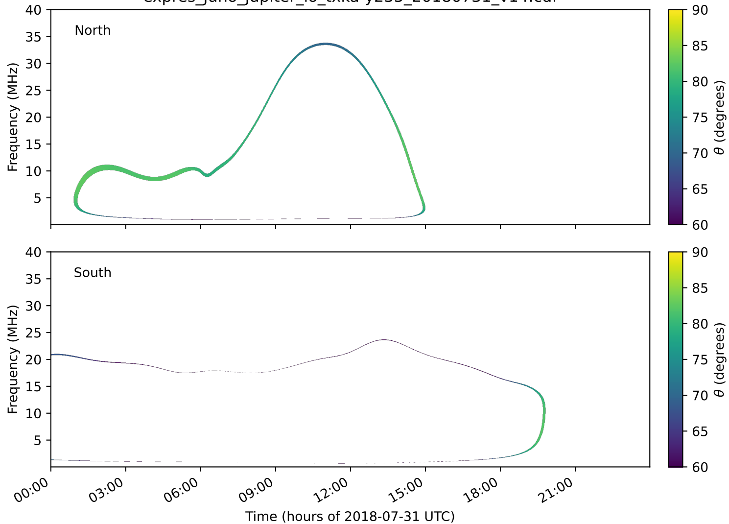
expres_juno_jupiter_io_txka-y235_20180731_v14.cdf
