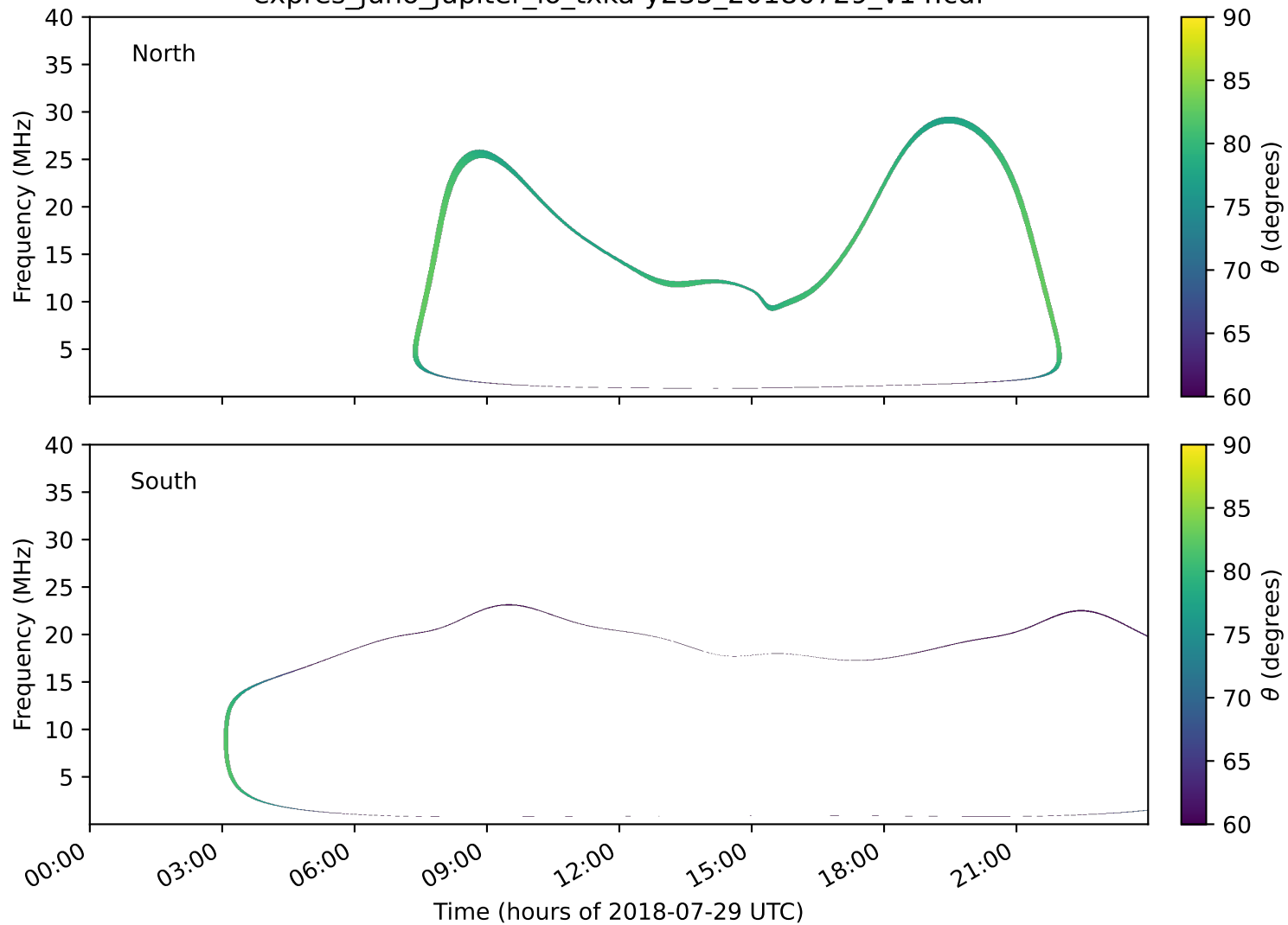
expres_juno_jupiter_io_txka-y235_20180729_v14.cdf
