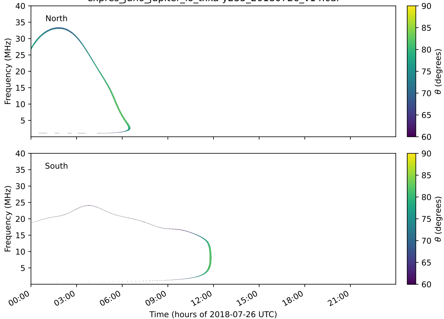
expres_juno_jupiter_io_txka-y235_20180726_v14.cdf
